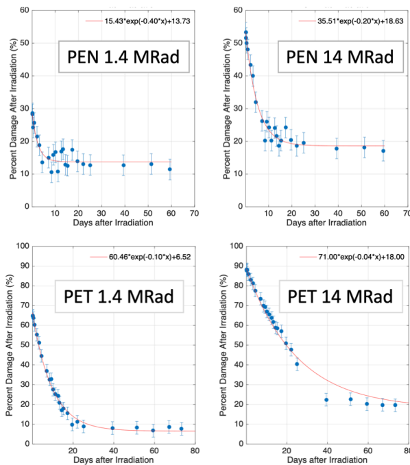
Figure 4. Percent damage after irradiation for PEN (top) and PET (bottom) samples that were irradiated to 1.4 MRad (left) and 14 MRad (right) for a duration of approximately two months.
