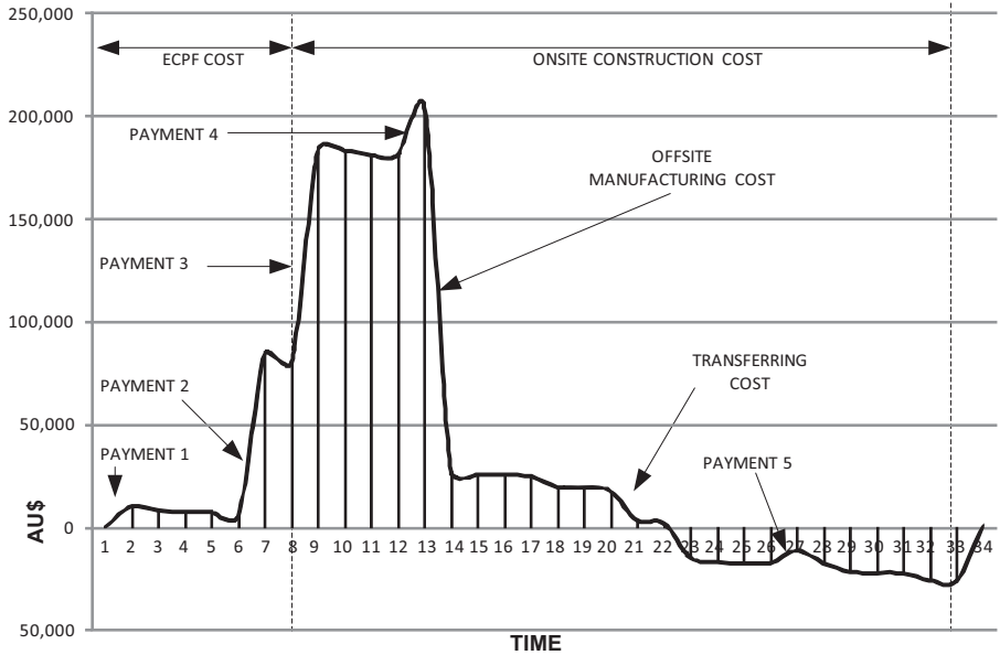
Figure 5. The net cash flow of Case 2
