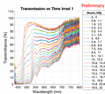
Figure 3. The transmission spectra of the blue fiber as a function of irradiation duration.
