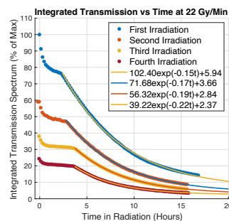
Figure 4. The integrated transmission vs. time for the four consecutive irradiation campaigns for the blue fiber.
