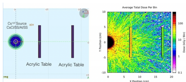
Figure 2. The displays from the Fluka simulation of the radioactive source and the sample holders.
