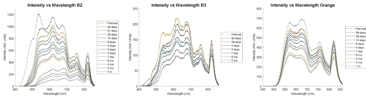
Figure 6. The absolute transmission spectra of blue (left), green (middle) and orange (right) fibers as a function of time after the first irradiation campaign.
