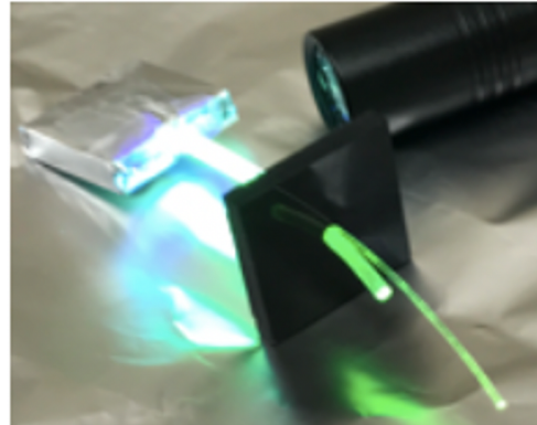
Figure 8. The picture of silicone (large) and Teflon AF (small) capillaries filled with silicone gel doped with 3HF.
