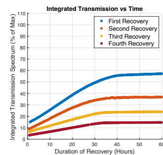
Figure 5. The transmission spectra integrals as a function of duration of recovery for the blue fiber.
