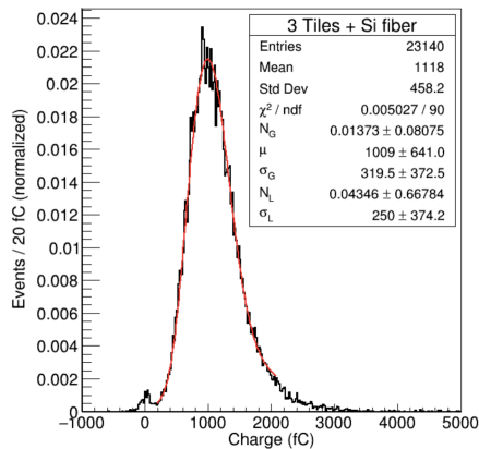
Figure 7. The charge distribution and the fit to Gaussian + Landau for the response of the 3 tiles + fiber assembly to 150 GeV muons.
